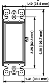
Dimensional Diagram
